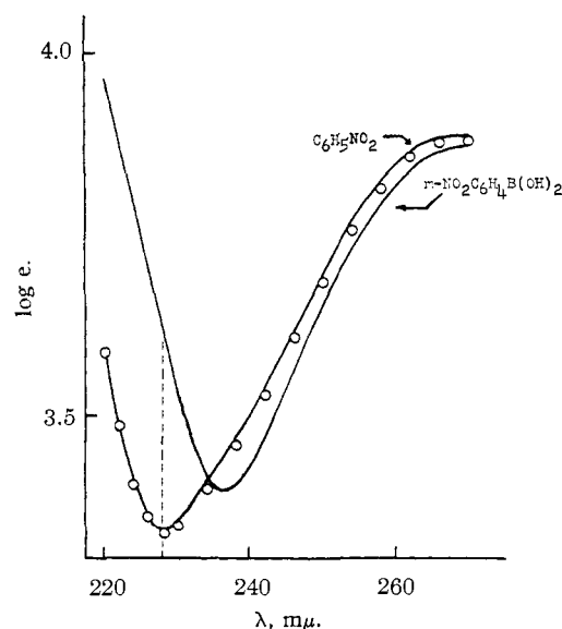
Fig. 2.—Absorption spectra of nitrobenzene and m -nitrobenzeneboronic acid. The dotted line is at 228 m \mu .
