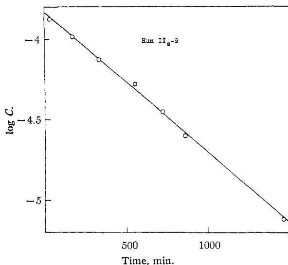
Fig. 1.—Rate plot for m -nitrobenzeneboronic acid; 60°, 97.0% H 2 SO 4 .
